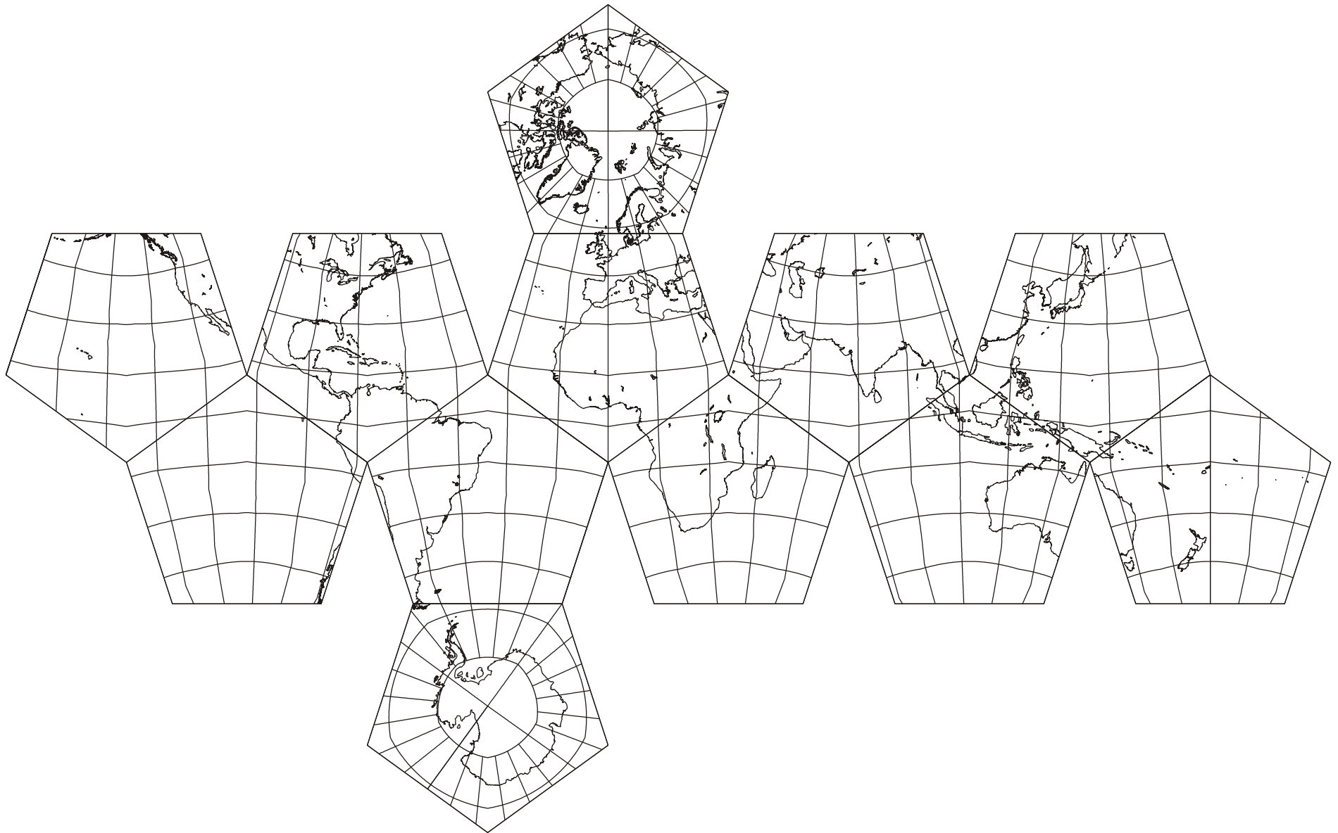
Equal-area Dodecahedron; Polyhedral Globe; Platonic Solid; Source: John Parr Snyder's Personal Software
