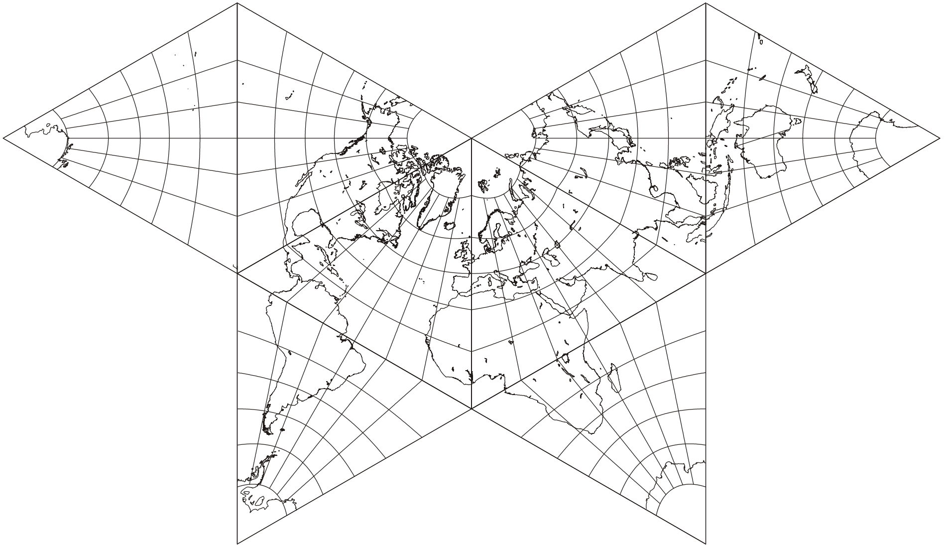
Gnomonic Octahedron; Polyhedral Globe; Platonic Solid; Source: John Parr Snyder's Personal Software
