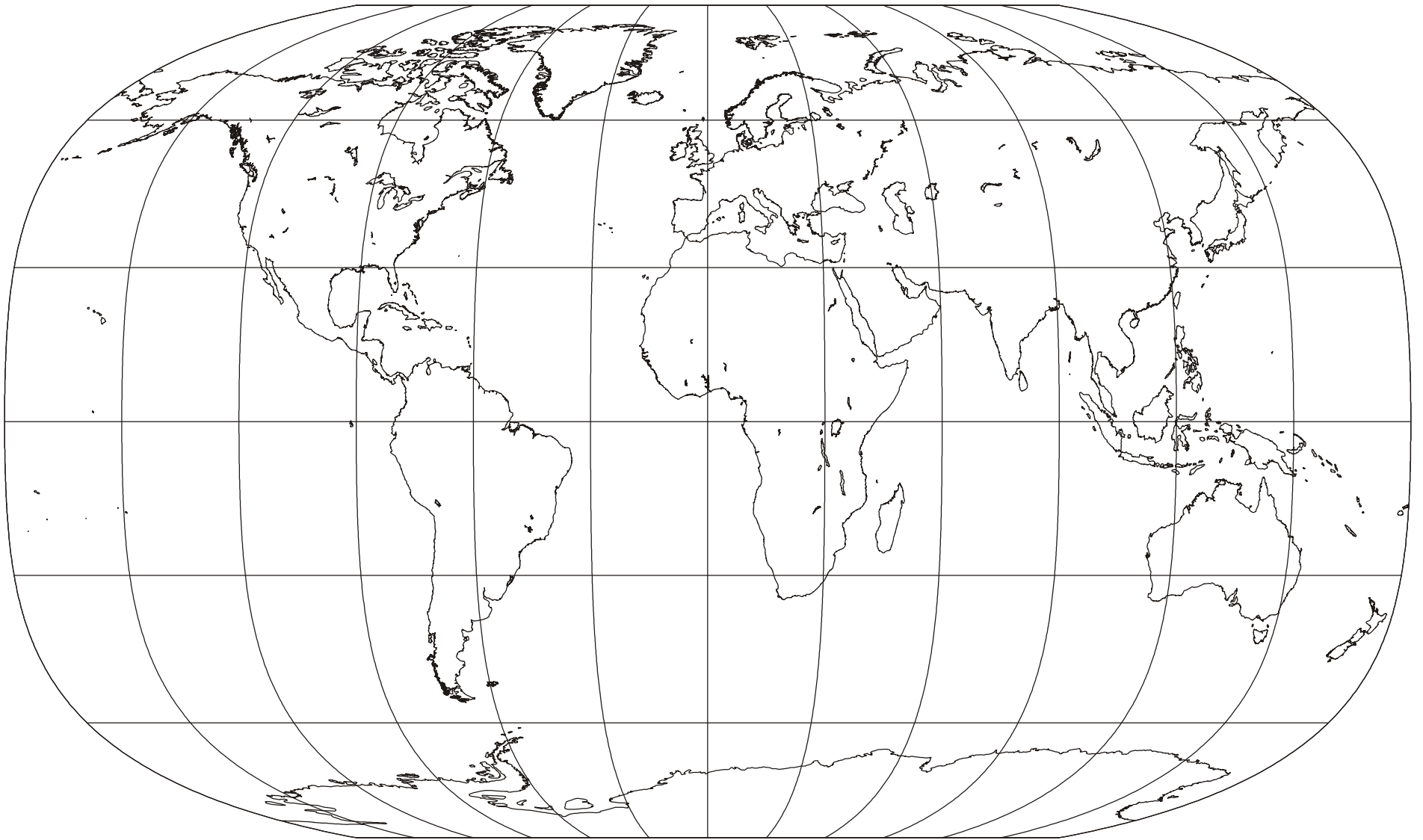
Canters Low-error Pseudocylindrical (b) projection; (with twofold symmetry and pole line half as long as the equator); Neither Conformal nor Equal-area; Frank Canters; 2002
