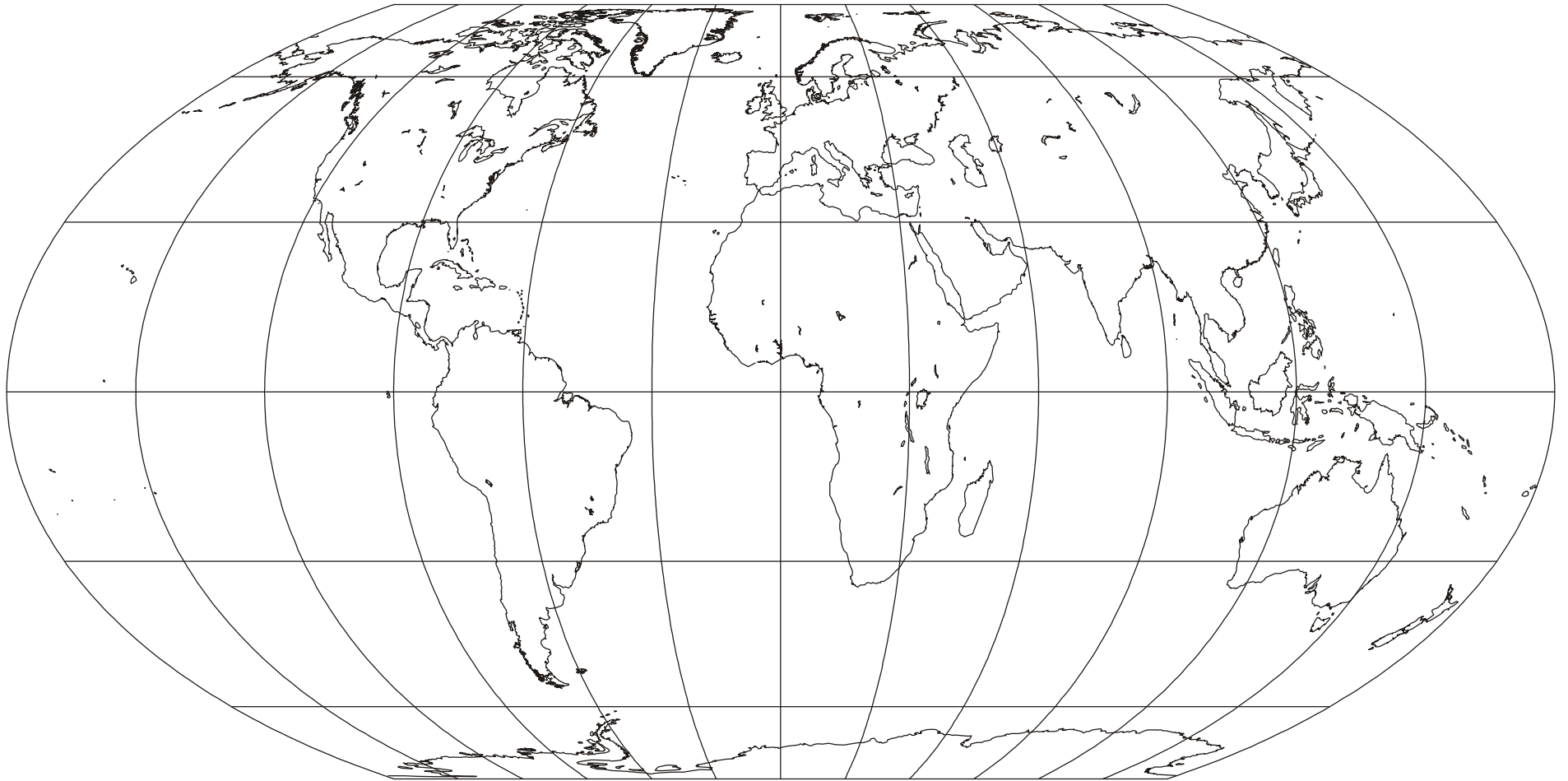
Wagner IV projection; Pseudocylindrical; Equal-area; K. H. Wagner; 1932; R. V. Putnins (P'2); 1934; W. Werenskiold (III); 1944
