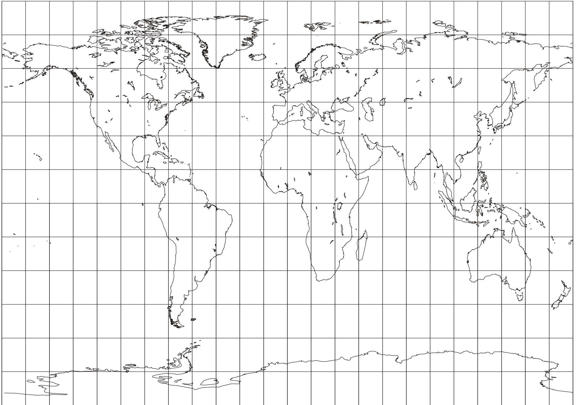
Gall Isographic (a Modified Equirectangular); Cylindrical; Neither Conformal or Equal-area; Standard Parallels = 45 Deg. N/S; James Gall; 1855
