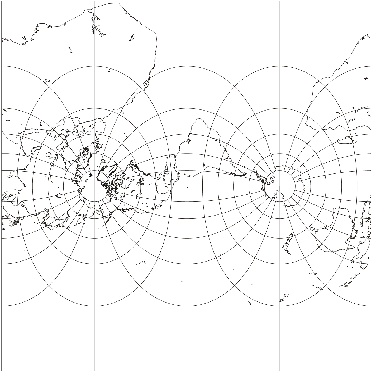
Transverse Mercator projection; Cylindrical; Conformal; Johann Heinrich Lambert; 1772
