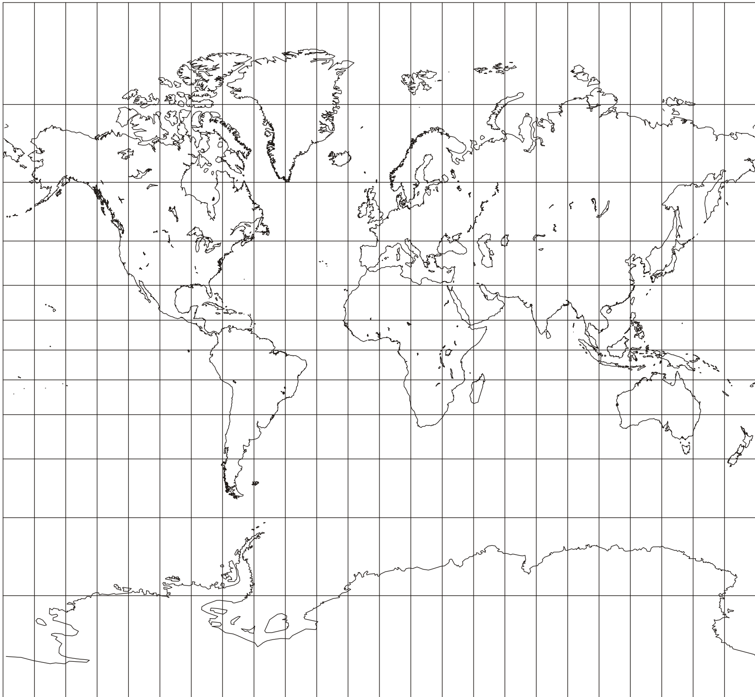
Urmayev 3 (Series approximation spaced parallels); Cylindrical; Not Conformal or Equal-area; N. A. Urmayev; 1947
