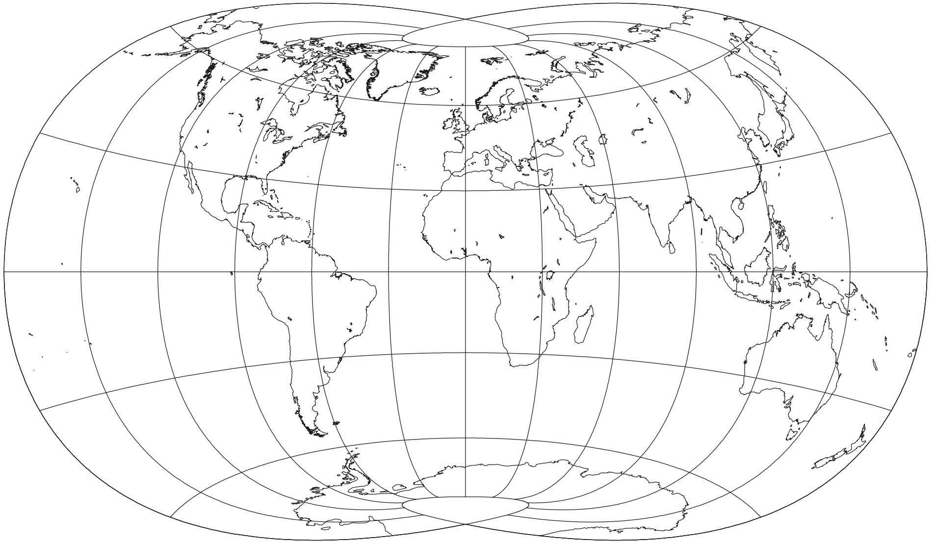
Laskowski Tri-Optimal Projection; Polyconic; Neither Conformal or Equal-area; P. H. Laskowski; 1991
