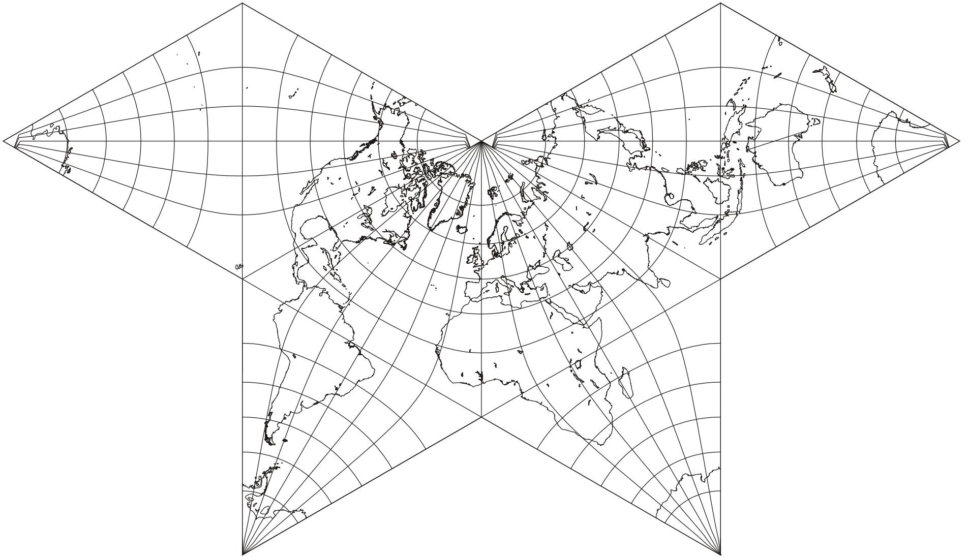
Conformal Octahedron; Polyhedral Globe; Platonic Solid; Source: Philip Voxland's 'World' Software
