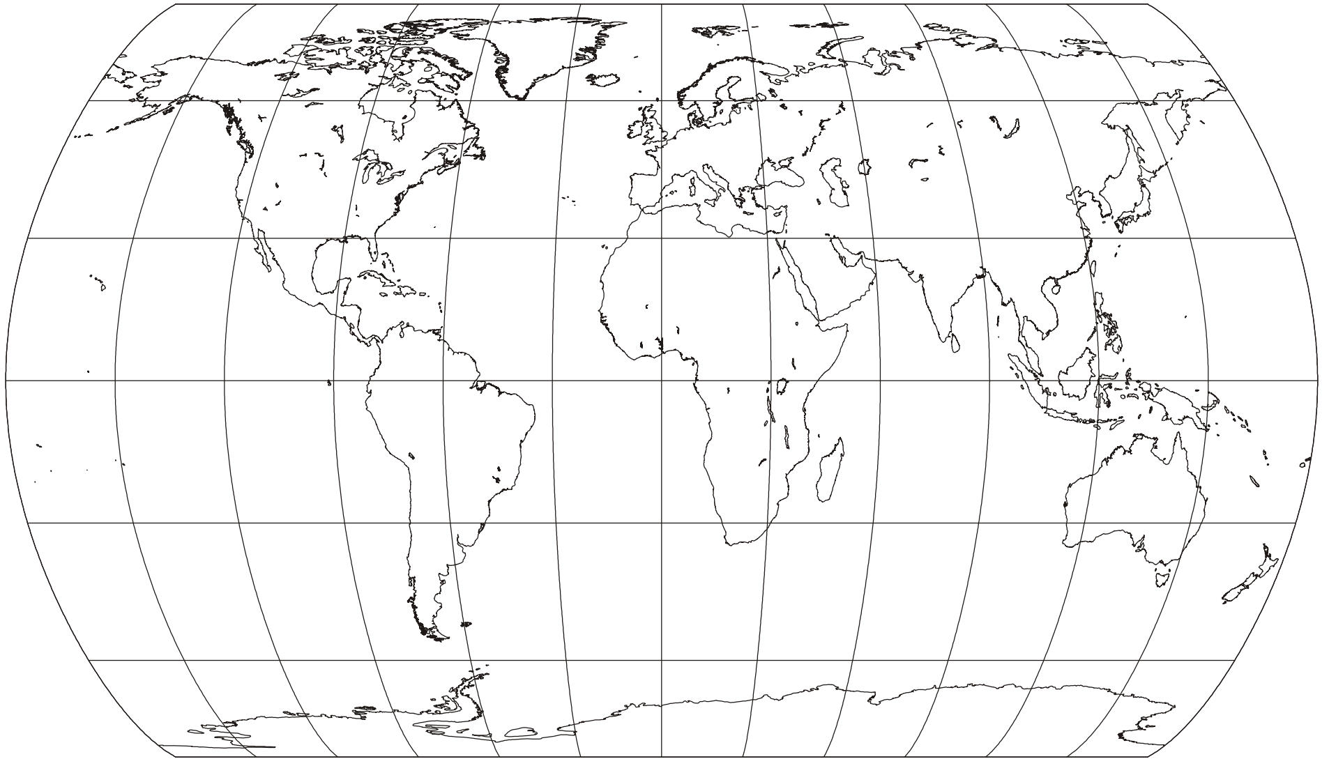
Canters Low-error Pseudocylindrical (a) projection; (With twofold symmetry); Neither Conformal nor Equal-area; Frank Canters; 2002
