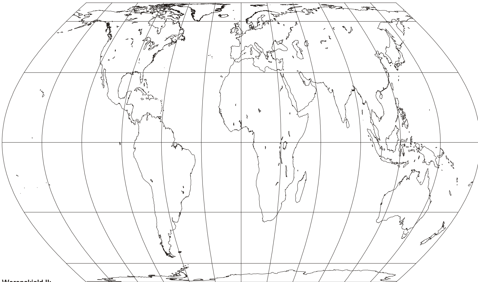
Werenskiöld II; Pseudocylindrical; Equal-area; Werner Werenskiöld; 1944/ 1945; K. H. Wagner (1); 1932; V. V. Kavrayskiy (VI); 1936
