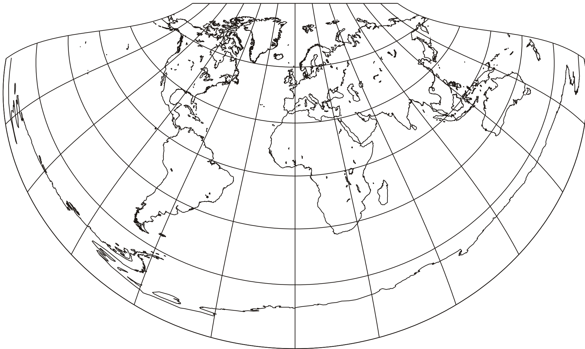
Seashell Projection
